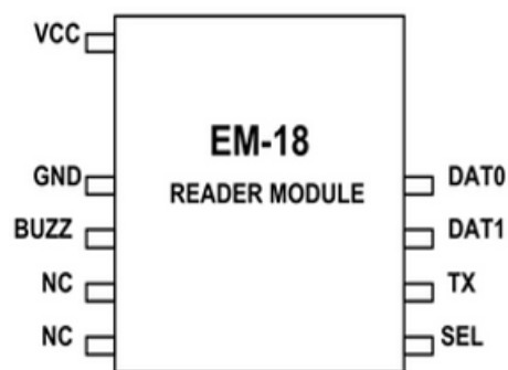
Fig. (3) Pin configuration of EM-18 RFID reader
