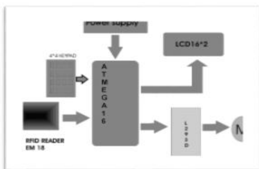
Fig. (7) Block Diagram of an RFID based security access control system
