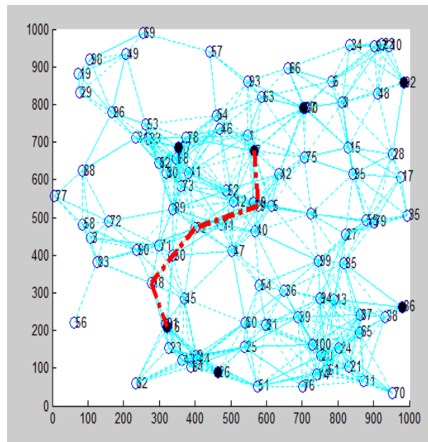
Fig 3.Black hole detection
