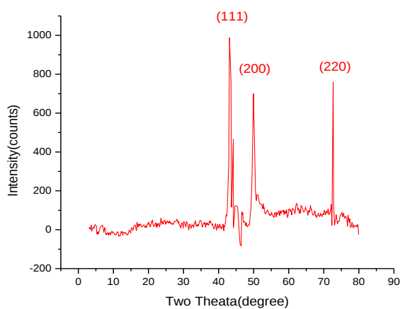
Figure -2 XRD pattern of electro deposited FeNiCo thin films with different concentration of Cobalt Sulphate.
