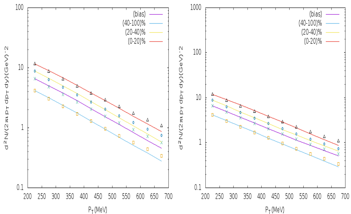
Fig5: Transverse momentum spectrum of \pi^- and \pi^+ for various centralities at \sqrt{s_{NN}}=200.0\text{GeV}
