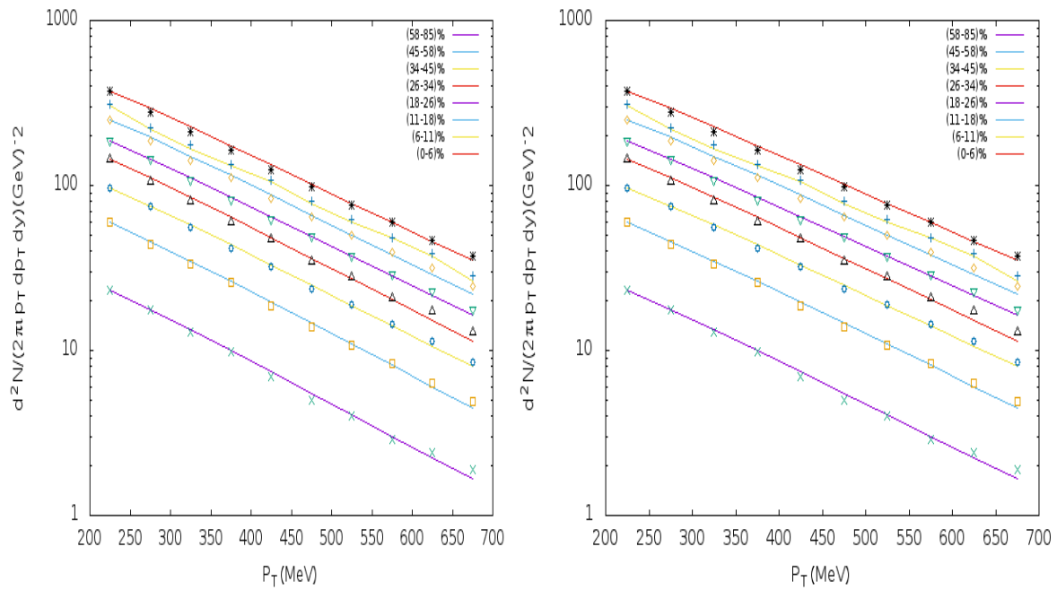
Fig4: Transverse momentum spectrum of \pi^- and \pi^+ for various centralities at \sqrt{s_{NN}}=130.0\text{GeV}
