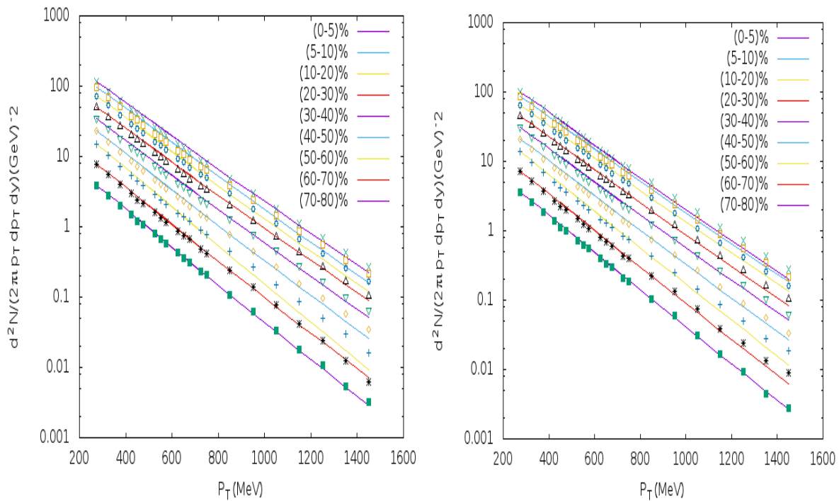
Fig1: Transverse momentum spectrum of \pi^- and \pi^+ for various centralities at \sqrt{s_{NN}} = 7.7 GeV
