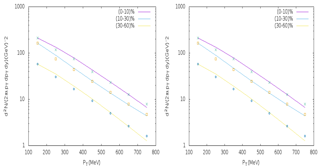
Fig 2: Transverse momentum spectrum of \pi^- and \pi^+ for various centralities at \sqrt{s_{NN}} = 9.2 GeV
