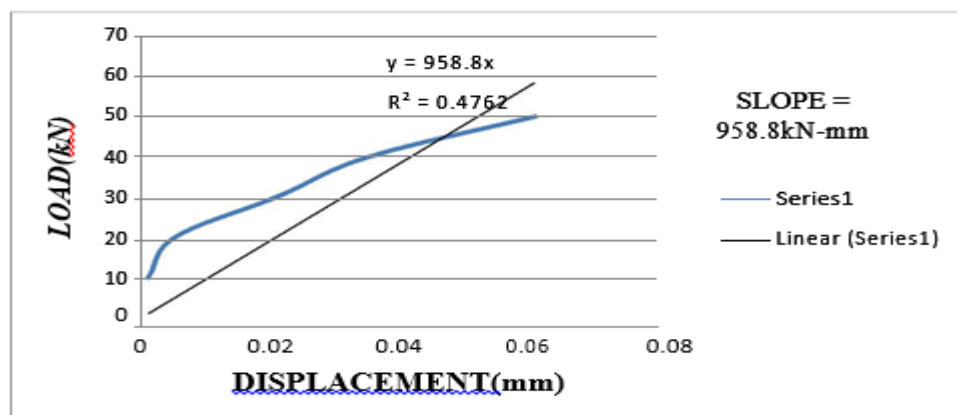
Fig 2.3 linear fit for C 1:1 (0 layers)
