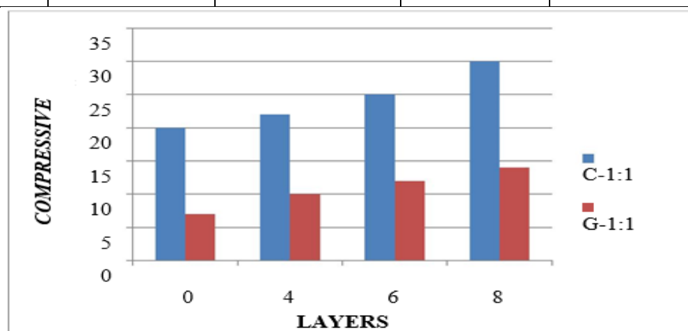
Graphical representation of compressive strength values with different layers for ratio 1:1.
