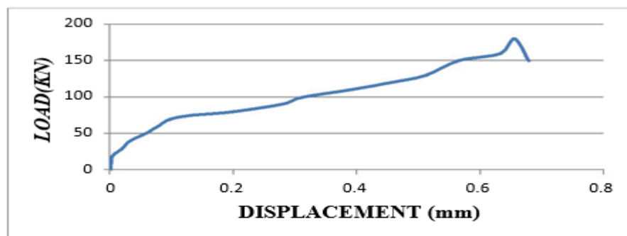
Fig 2.2 Graphical representation of load-displacement for C 1:1 (0 layers).
