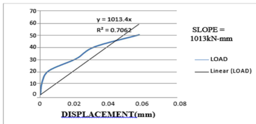
Fig 1.3 linear fit for C 1:1.5(0 layers).
