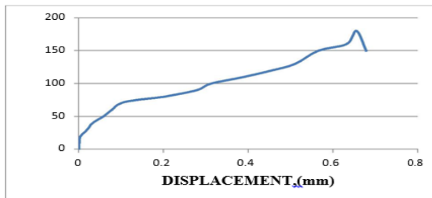
Fig 2.2 Graphical representation of load-displacement curve for C 1:1.5(0 layers).
