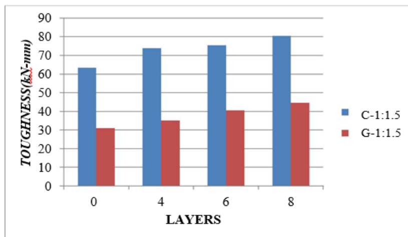
Graphical representation of toughness with no.of layers for ratio 1:1.5.
