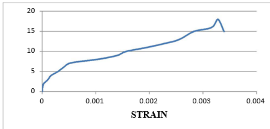
Fig 2.1 Graphical representation of stress-strain curve for C 1:1.5(0 layers).
