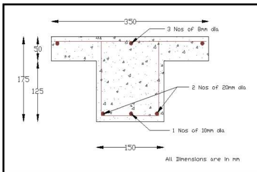
Figure 1: Detailing of Reinforcement [14]
