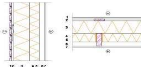
Fig. 3. ZEB wall composition: 1 – gel coating; 2 –ventilated gap; 3 – slab SPU AL 150 mm; 4 – slab SPU AL 100 mm; 5 – rack wooden frame; 6 –space for laying of engineering communications; 7 –interior finishing layer.
