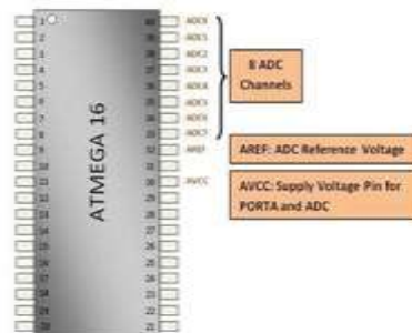
Fig 4. ATMEGA 16 microcontroller
