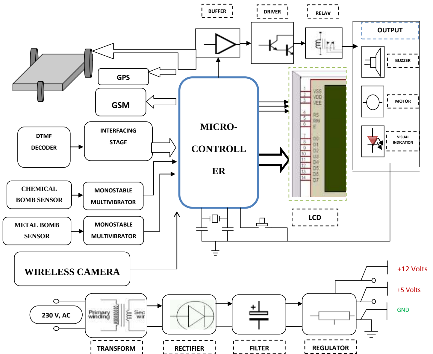
Fig 1. Block Diagram of Land Rover Robot.
