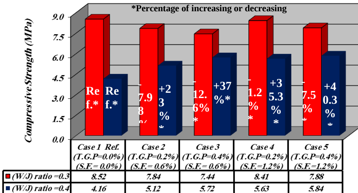
Bar Chart (1): Combined Effect of T.G.P. and S.F. Contents on Compressive Strength of Juss For (W/J) Ratio = (0.3) And (0.4) .
