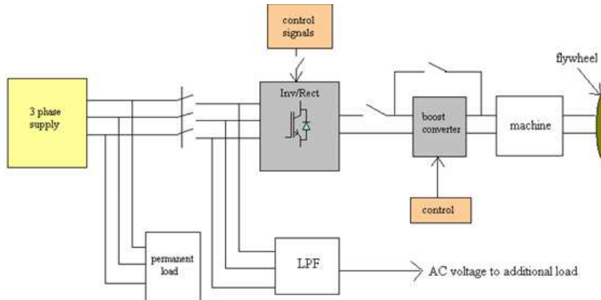
Figure. 1 Block Diagram of The Flywheel Energy Storage System (FESS)
