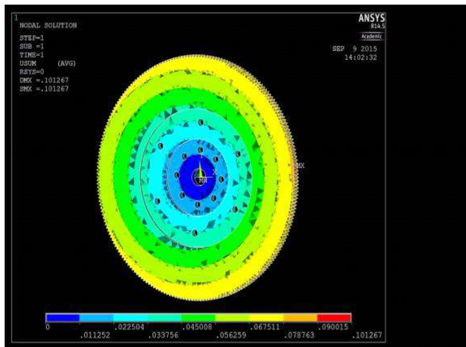
Figure. 6 Displacement Vector Sum
