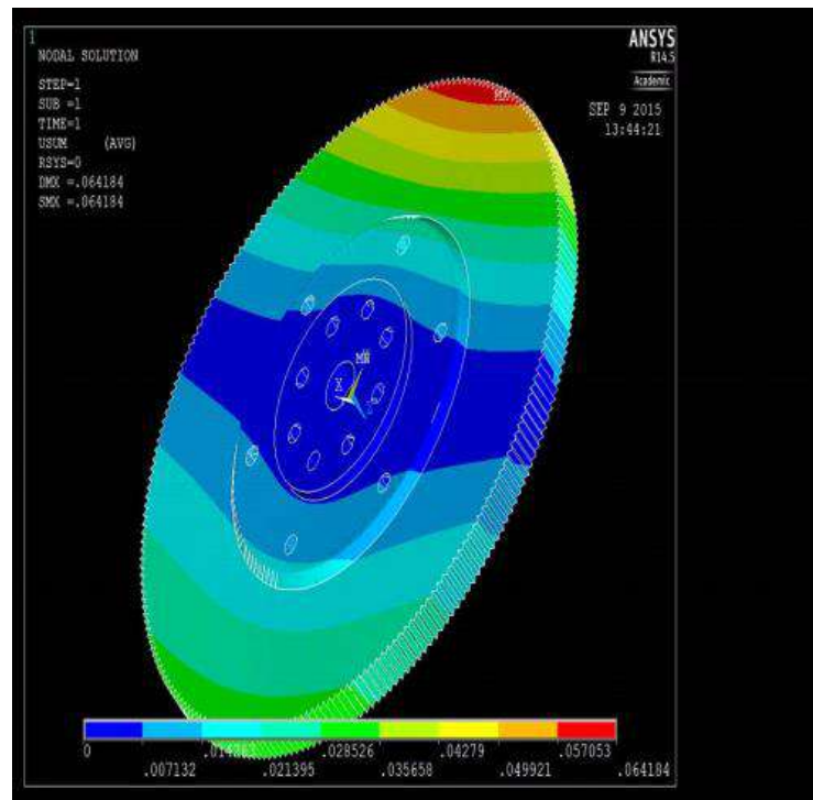
Figure. 9 Displacement Vector Sum
