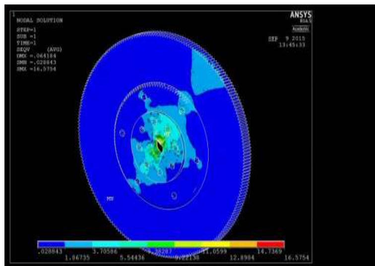
Figure 10 Vonmises Stresses
