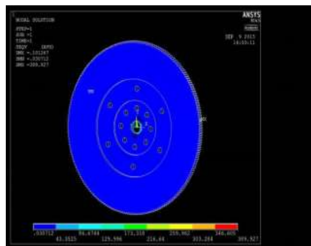
Figure 7 Vonmises Stresses
