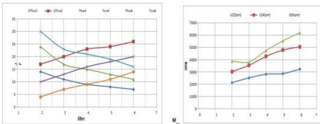
Fig 4 change in temperature of hot and cold water with varying flow rate of hot water
