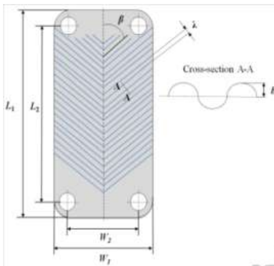
Fig 1 corrugated plate
