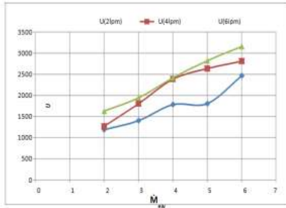
Fig 6 shows the variation of overall heat transfer coefficient with mass flow rate of hot water.
