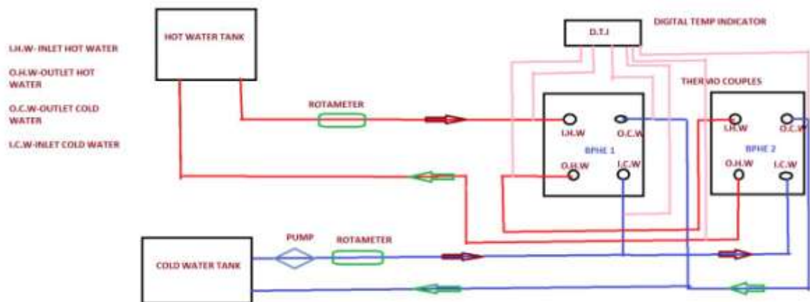
Fig 2. Schematic diagram of my experimental setup
