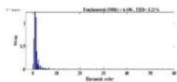
Fig 14. Neutral wire current
