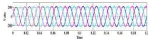
Fig 11. 3-phase source voltages
