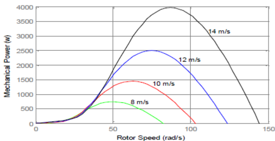
Figure4: The Torque curves for different wind speeds and zero pitch angle
