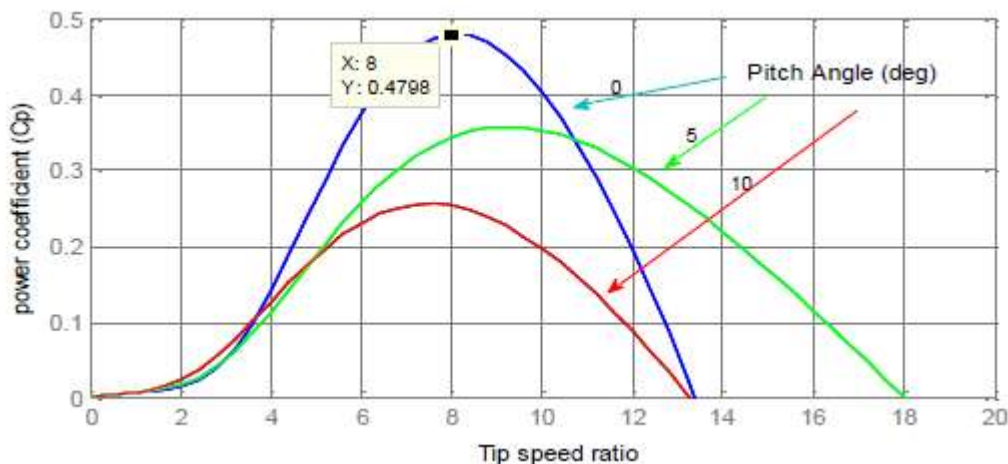
Figure 3: Power coefficient characteristics of a wind turbine.
