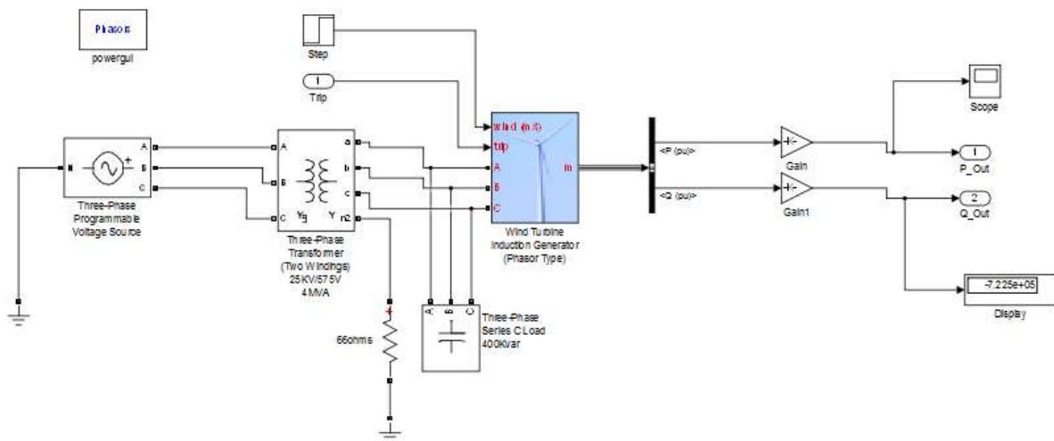
Fig 5. Simulation diagram of Wind Turbine
