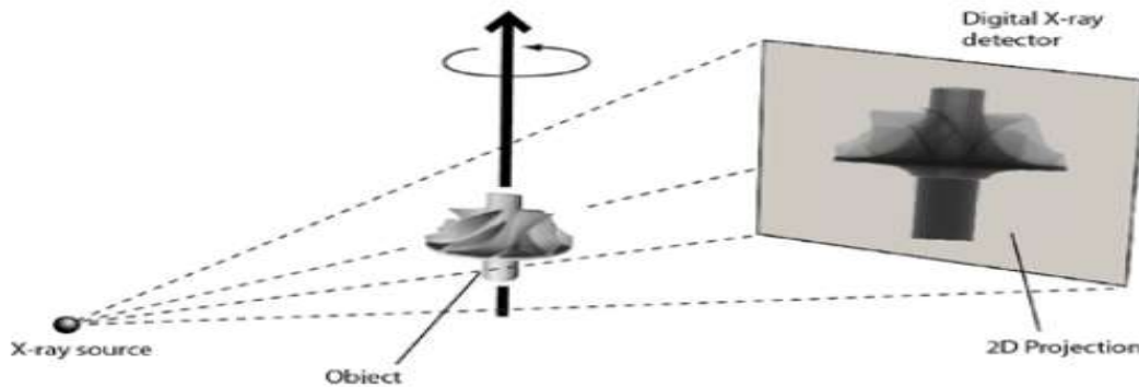
Fig.1: Working of CT Scanning [3]
