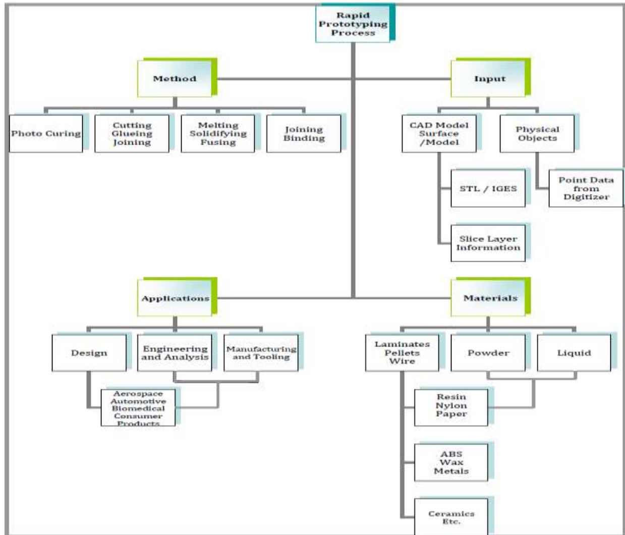
Fig.7:Overview of RP Process [13]
