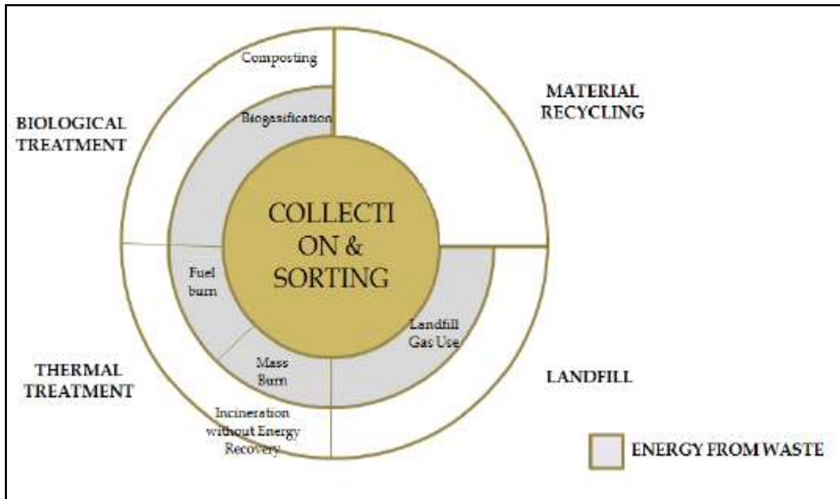
Figure-6: Elements of Integrated Solid Waste Management [41]
