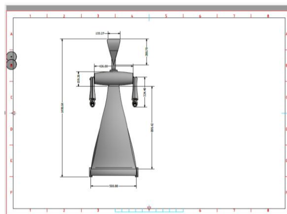
Fig. 8: Drafting of serving robot
