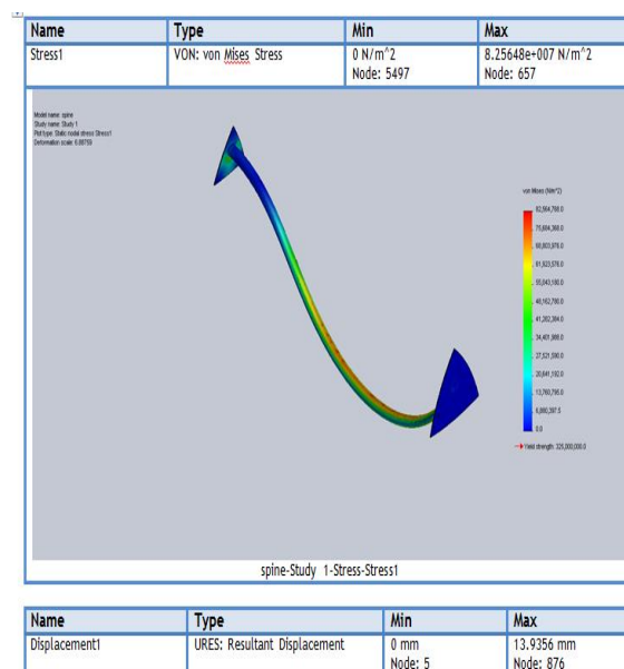
Fig. 6: Stress Analysis of Spine
