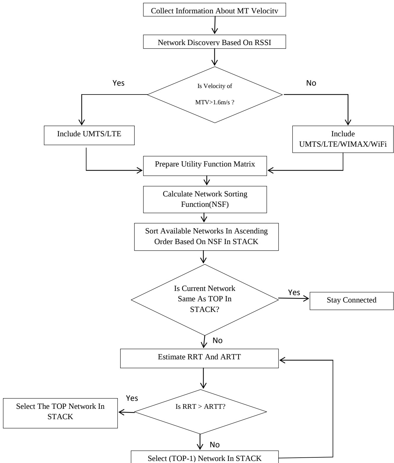
Fig. 2. Algorithm for Proposed Network Handover Scheme
