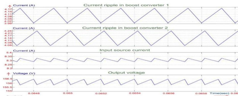
Fig. 2. Ripple waveforms of 2-phase IBC
