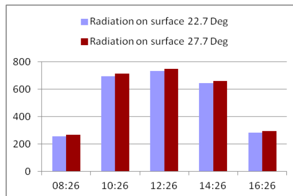
Figure 7. The amount of radiation incident on the surface of the PV system with 22.7 Deg and 27.7 Deg of tilt for the same horizontal radiation data on Dec 24, 2008.
