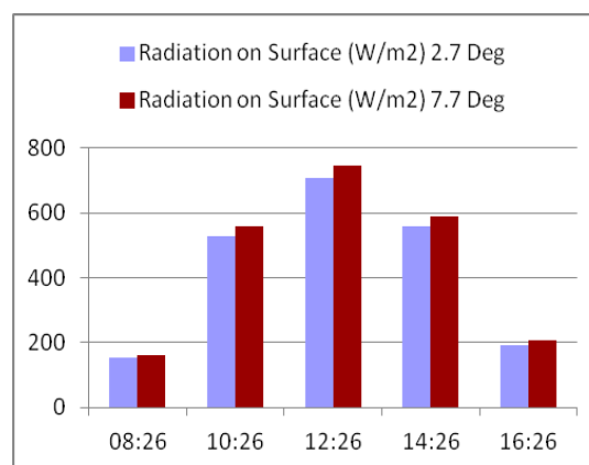
Figure 4. The amount of radiation incident on the surface of the PV system with 2.7 Deg and 7.7 Deg of tilt for the same horizontal radiation data on Dec 23, 2008.
