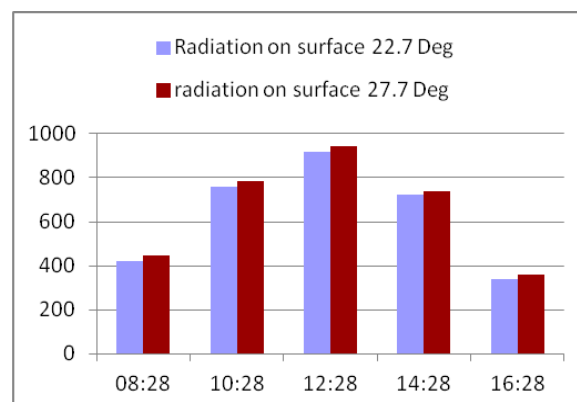
Figure 8. The amount of radiation incident on the surface of the PV system with 22.7 Deg and 27.7 Deg of tilt for the same horizontal radiation data on Dec 27, 2008.
