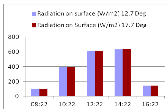
Figure 5. The amount of radiation incident on the surface of the PV system with 12.7 Deg and 17.7 Deg of tilt for the same horizontal radiation data on Dec 15, 2008.
