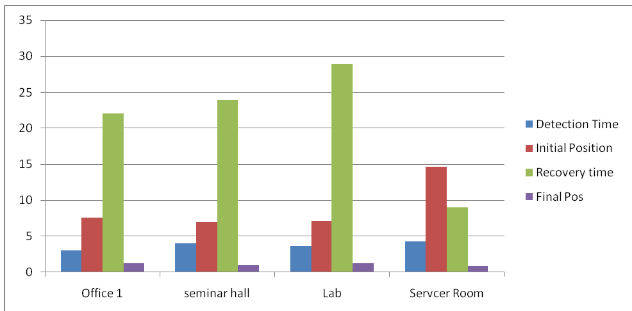
Figure 2 : Localization failure recovery
