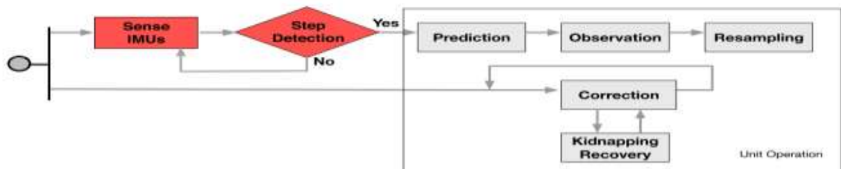
Figure 1 : Proposed System Architecture
