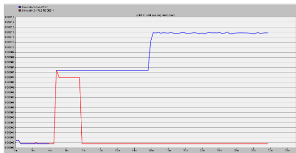
Fig. 7. Delay when traffic is rerouted using TE technique
