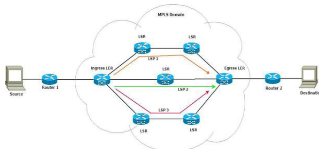
Fig. 1. Simple MPLS network.
