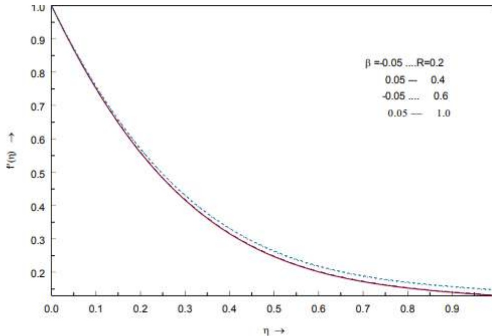
Fig 6 Effect of radiation parameter for various values of heat source/sink in PST case with Pr=7.0 , E=0.02 , K1=0.1 , K2=0.2 for velocity profile
