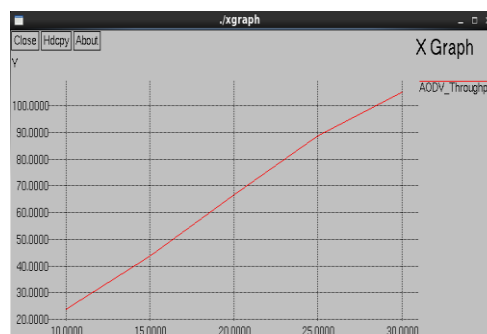
Fig 5: Analyzing number of nodes against through-put
