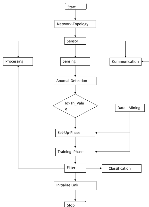
Fig 3 : Flowchart of mIDS system
