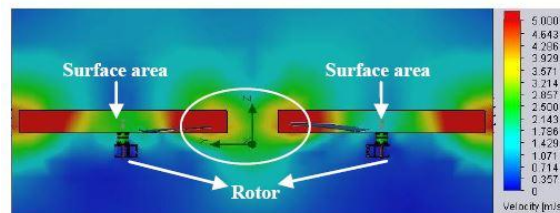
Fig. 8 Isosurface airflow between propellers with 9880(rpm)
