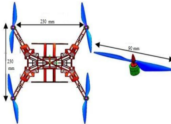
Fig.1. Body frame quad copter model
