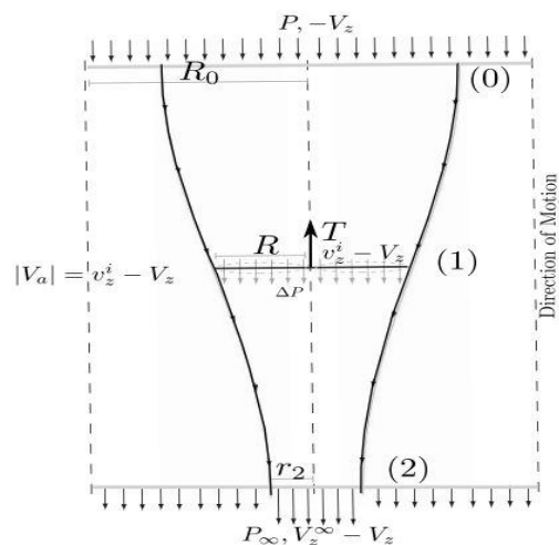
Fig. 3. Vertical stream tube for hover and axial analysis.
