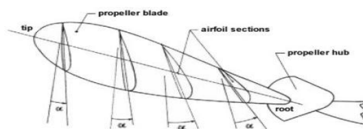
Fig. 5 Fixed pitch propeller geometry
