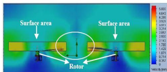
Fig. 9 Isosurface airflow between propellers with 6240 (rpm)
