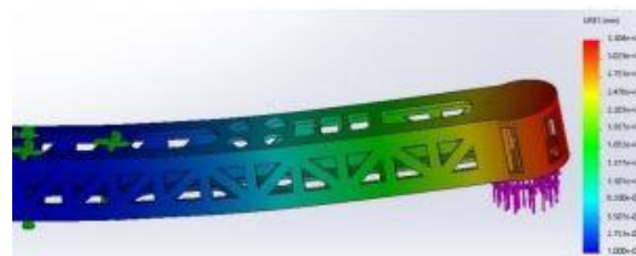
Fig. 2. Wing frame displacement analysis
