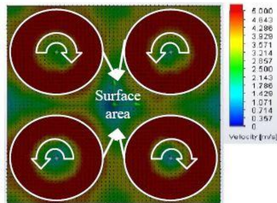
Fig. 7 Isosurface airflow around propeller
