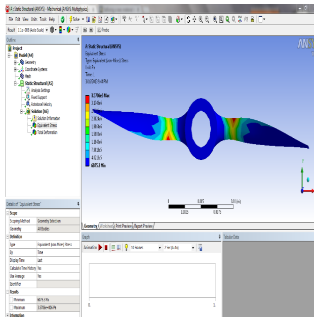
Fig.11 Analysis of Propeller
