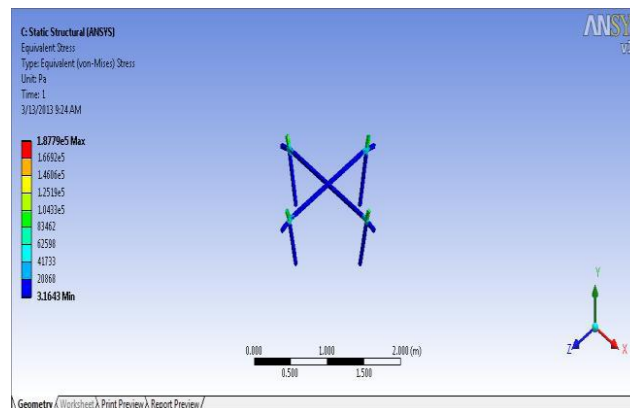
Fig.10. Analysis of Quadcopter Frame
