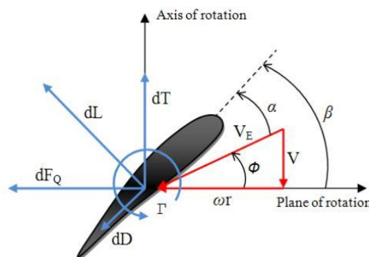
Fig. 6. Vector diagram for a section dr at length r away from centre of the propeller
