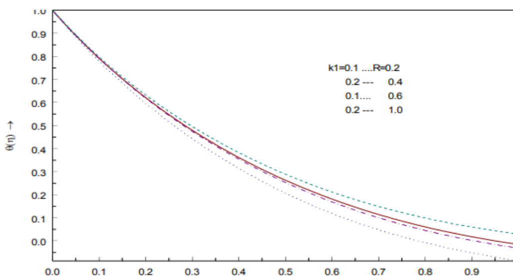
Fig.1 Effect of radiation parameter for various values of K_1 in PST case with Pr=7.0 , E=0.02 , K_2=0.0 , B=-0.05 for temperature profile
