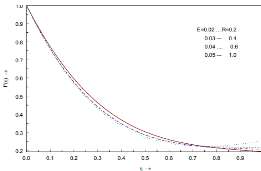
Fig.5 Effect of radiation parameter for various values of Eckert number in PST case with Pr=7.0 , B=-0.05 , K1=0.1 , K2=0.2 for velocity profile
