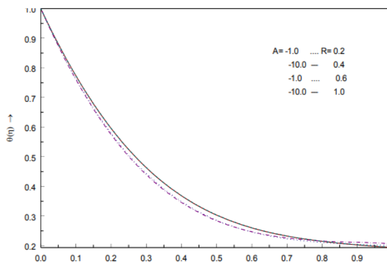
Fig.3 Effect of radiation parameter for various values of A in PST case with Pr=7.0 , E=0.02 , K1=0.1 , K2=0.2 , B=-0.05 for temperature profile
