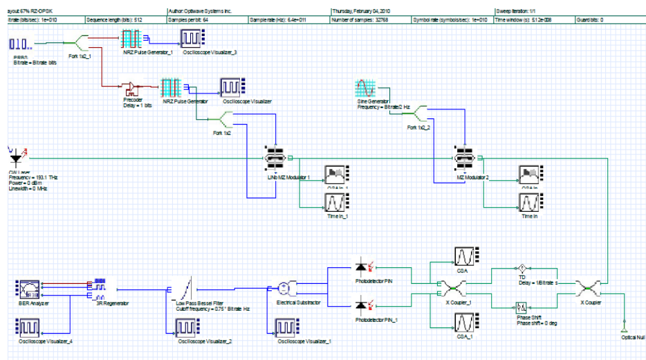
Fig 2. Design of RZ-DPSK modulation
