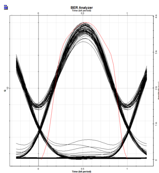
Fig 5. Eye diagram of the RZ-DPSK
