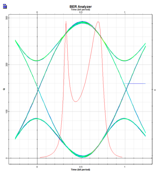
Fig 4. Eye diagram of the CSRZ-DPSK
