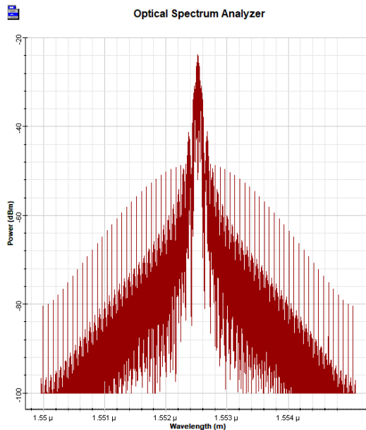
Fig 6. Optical spectrum of RZ-DPSK
