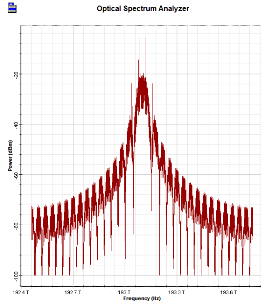
Fig 7. Optical spectrum of CSRZ-DPSK
