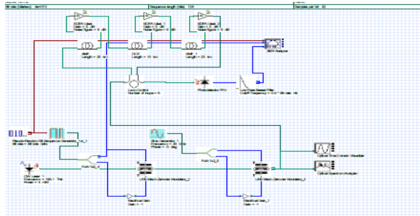
Fig 3. Design of CSRZ-DPSK modulation
