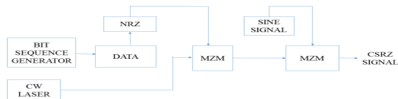
Fig 1. Block Diagram for Generation of Carrier Suppressed Return-to-Zero (CSRZ) signal
