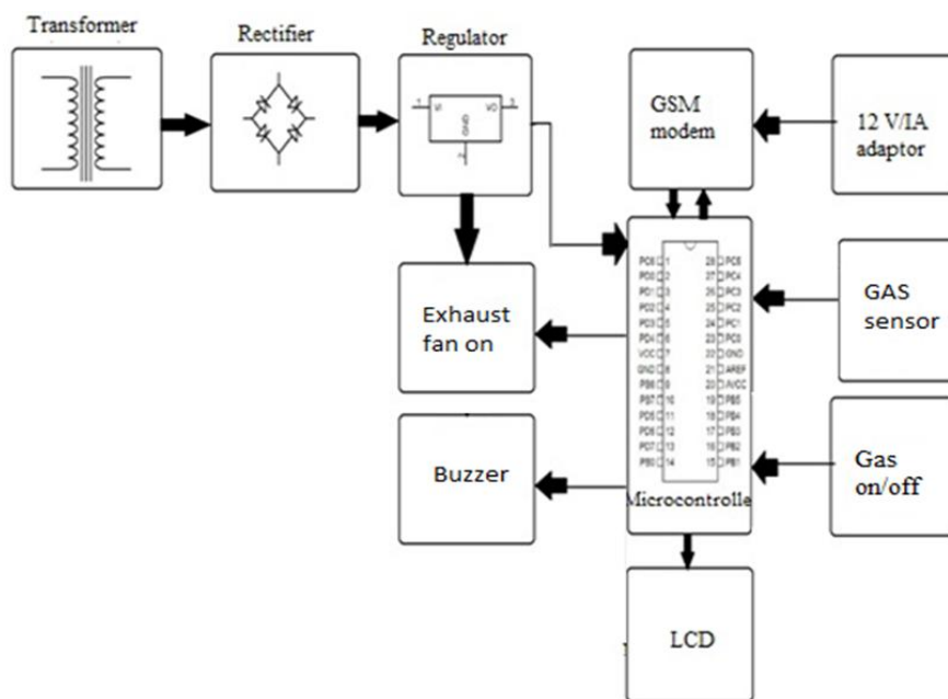
Figure 1: Proposed Model
