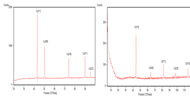
Fig. 4.1.1 XRD Pattern Of Cu (1) & Cr (2) powder
