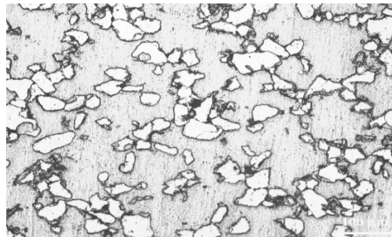
Fig 4.5.3 Optical micrographs of annealed CuCr30 a) as received b) 2 hrs. Ball milled c) 6.5 hrs. Ball milled Cr powder. Fig.4.5.3 shows that grain growth occurred during annealing which softens the material increasing its electrical conductivity
