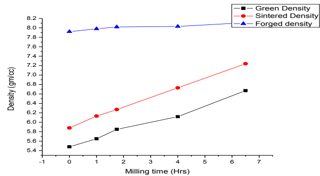
Fig 4.2.1 Variation in different densities with milling time
