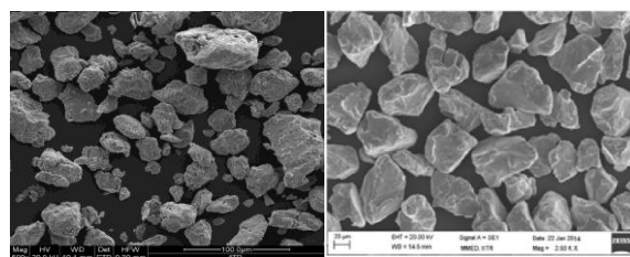
Fig. 4.1.2 SEM Image Of Cu (1) & Cr (2) powder
