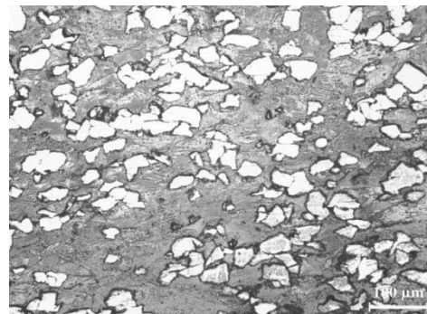
Fig 4.5.2 Optical Micrographs of sinter-forged CuCr30
