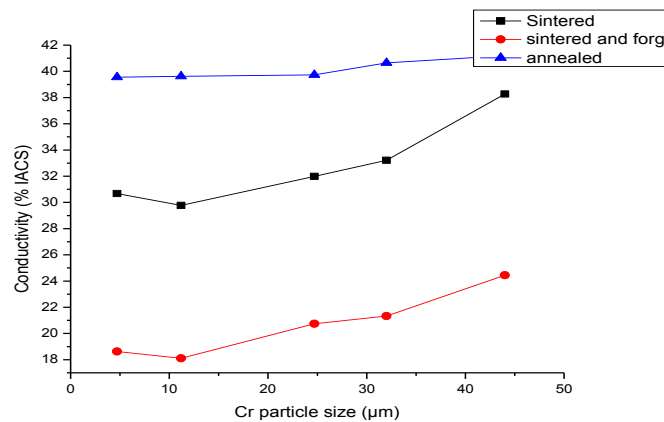
Fig 4.4.1 Conductivity of various samples Vs Cr particle size
