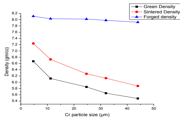
Fig 4.2.2 Variation in different densities with Cr particle size
