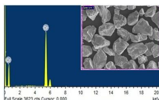
Fig 4.1.4 EDS analysis
