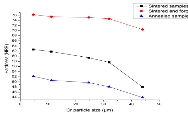
Fig 4.3.1 Hardness of different samples Vs. Cr particle size
