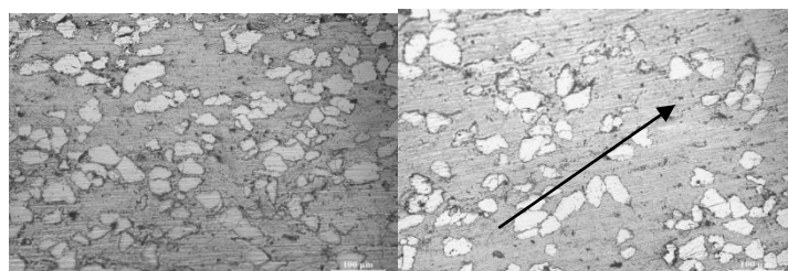
Fig 4.5.4 Sinter-forged CuCr30 in longitudinal (left side) and transverse plane (right side)
