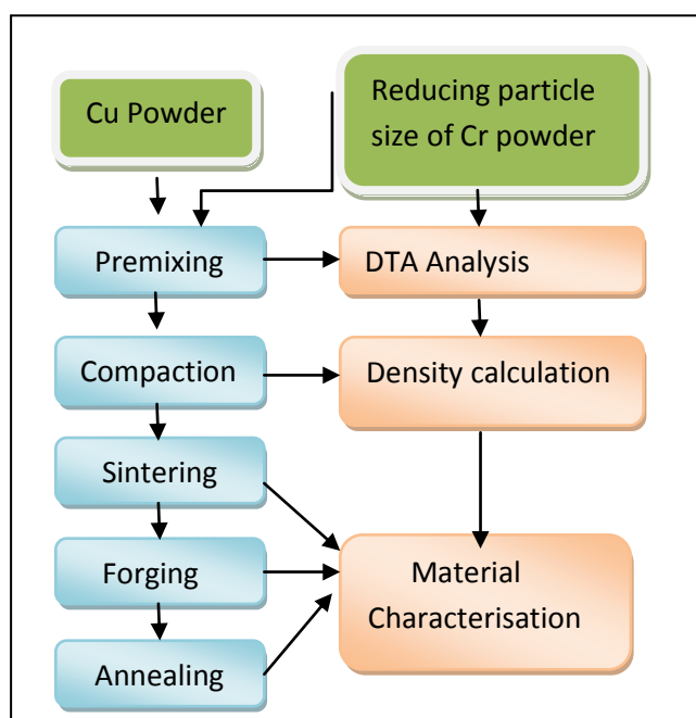
Fig 3.1.1 Typical Flow chart for experimental work
