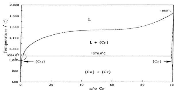
Fig 2.1 Cu-Cr phase diagram [10]
