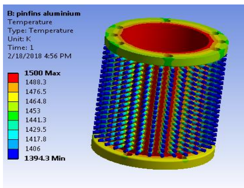
Fig 3.12 Temperature distribution
