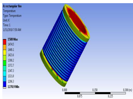
Fig 3.8 Temperature distribution
