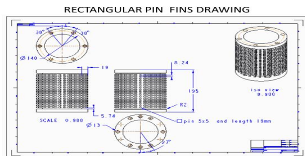
Fig2.7 part drawing of cylinder
