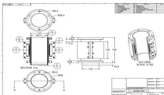
Fig2.6 Assembly drawing of engine cylinder
