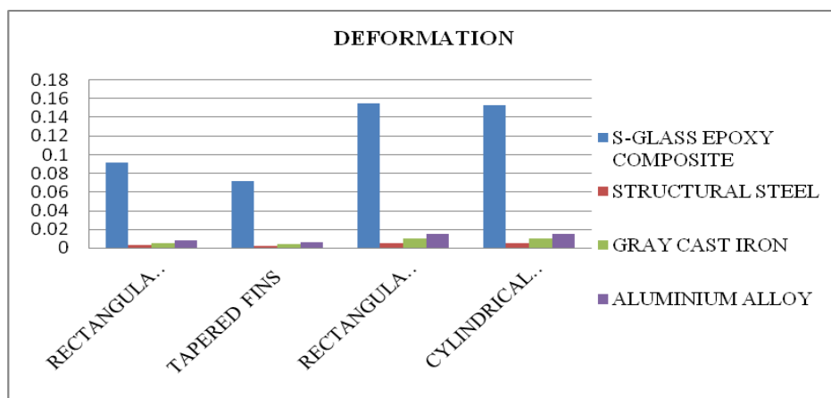
5.4 The graph shows the variations of deformations of various geometries and materials
