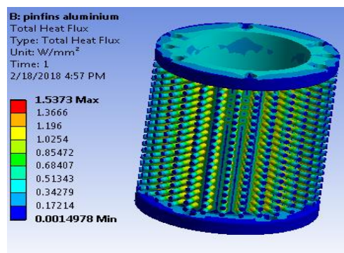
Fig 3.13 total heat flux
