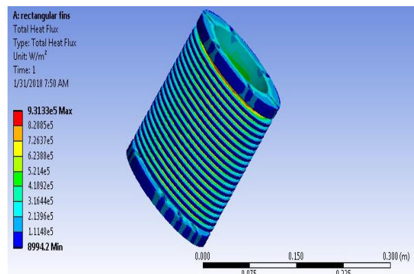
Fig 3.9 total heat flux
