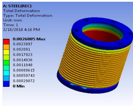
total deformation
