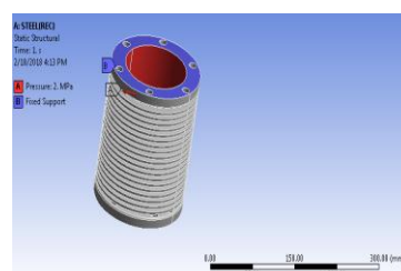
Fig 3.4 boundary conditions
