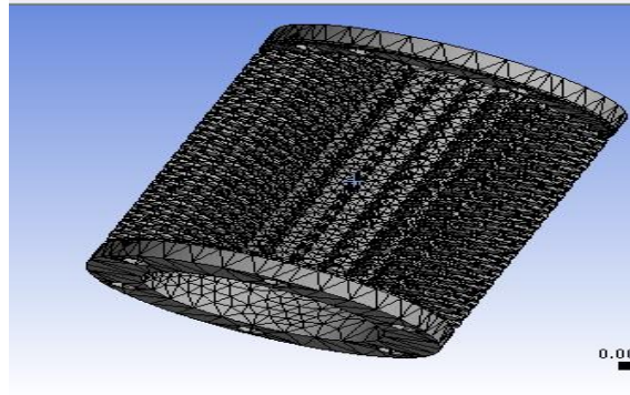
Fig 3.11 meshing
