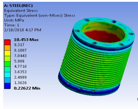
Fig 3.6 von-misses stresses
