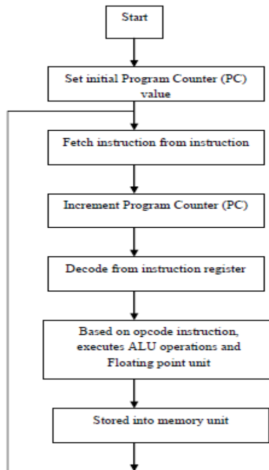
Fig.5 Flow Chart of Proposed Processor
