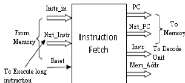
Fig.2 I-Fetch Unit
