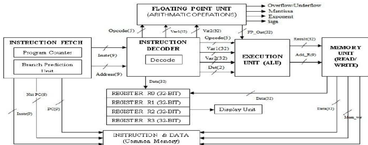
Fig.1 Architecture of 32-bit RISC Processor with FPU
