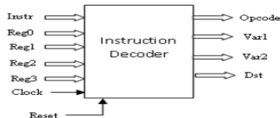
Fig.3 Instruction Decoder Unit
