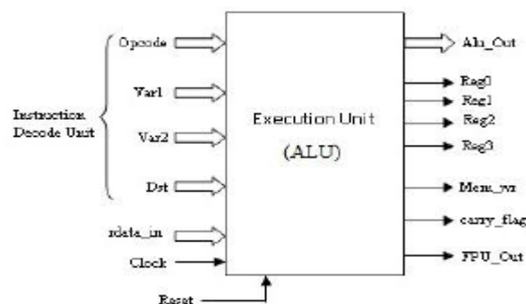
Fig.4 Execution Unit
