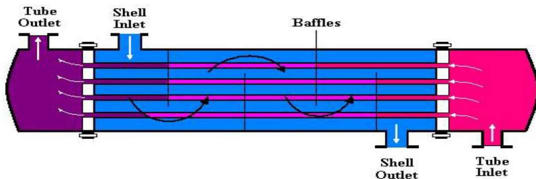
Fig1: Shell-and-tube heat exchanger
