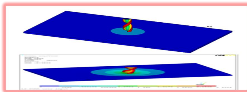
Fig.11 delamination at entry and exit modelled by Teja et al. [17].
