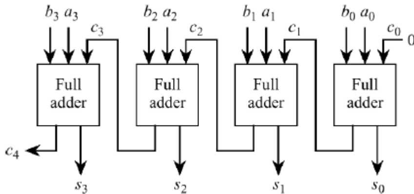
Figure 3 Ripple Carry Adder
