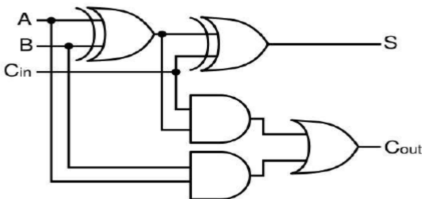
Figure 2 Full adder logic design
