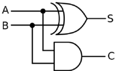
Figure 1 Half adder logic diagram
