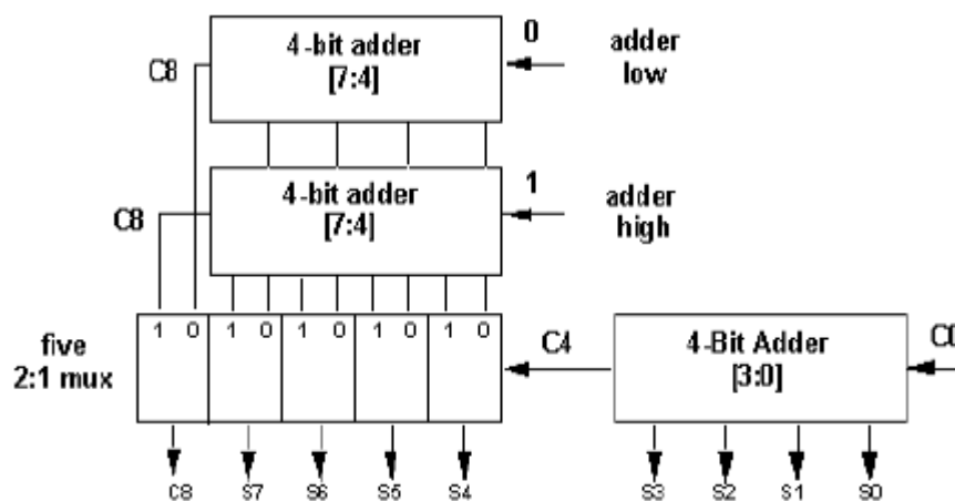
Figure 4 Carry Select Adders
