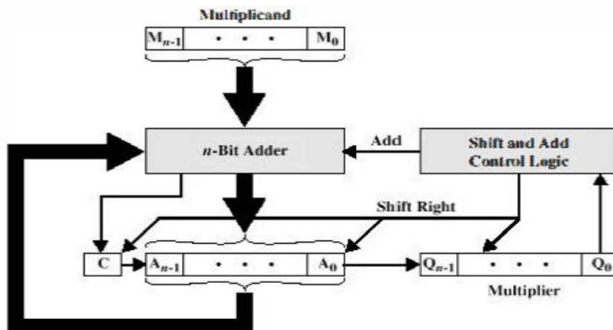
Figure7. Multiplier of two n-bit values.
