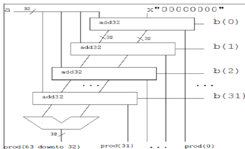
Figure 6. A partial schematic of the multiplier
