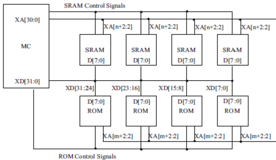
Figure 4: Memory system architecture
