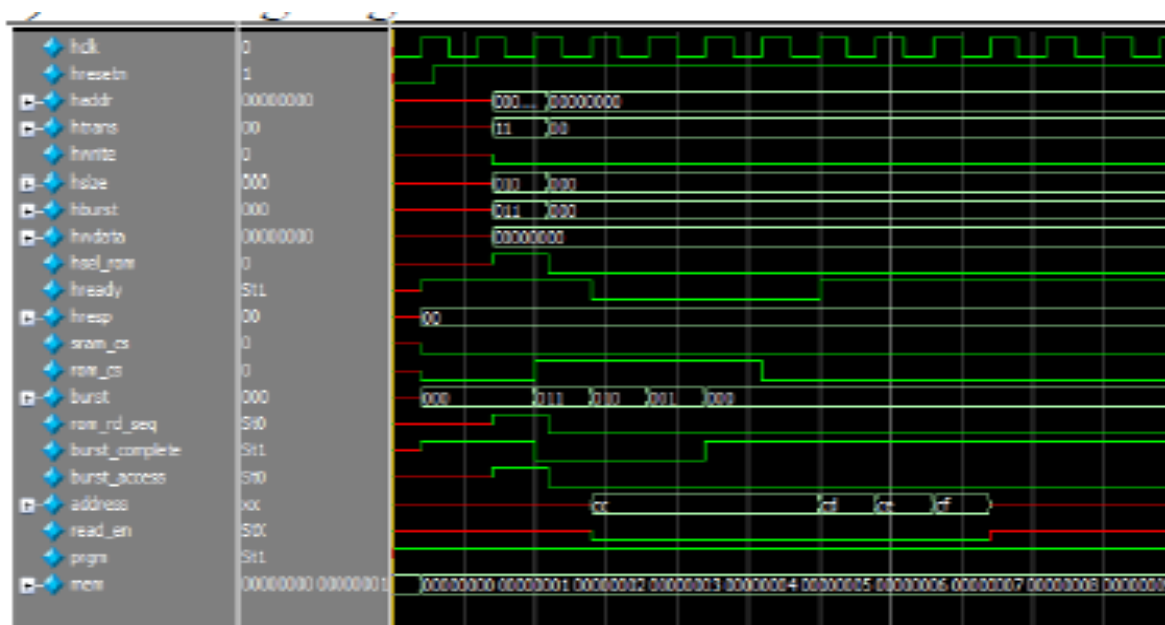
Fig 5. Read with zero wait state from ROM
