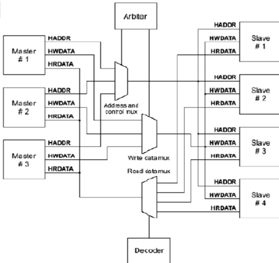
Figure 1: AMBA AHB Block diagram
