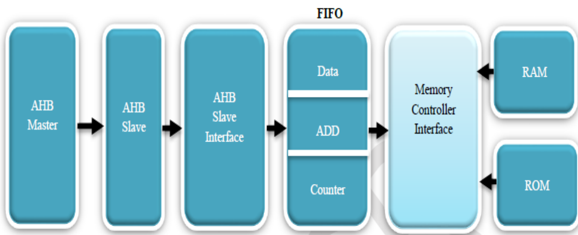
Figure 2. Top architecture of AHB memory controller
