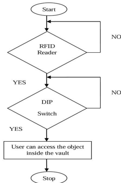
Fig.4 Flow chart-Working of Secondary Authentication
