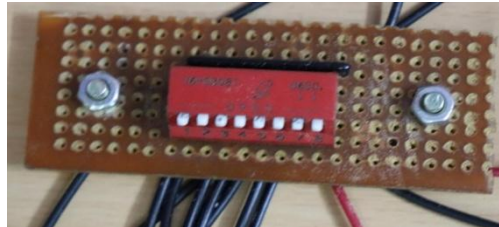
Fig.14 DIP Switch
