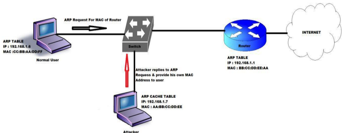
Fig. 1 ARP Request and ARP Reply
