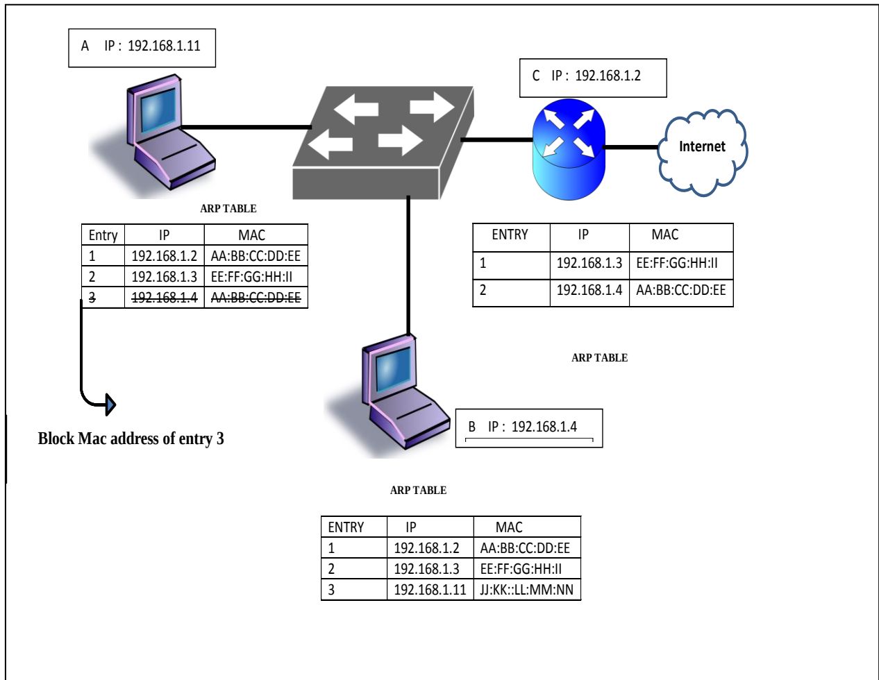
Fig. 4 Prevention from ARP Spoofing Attack
