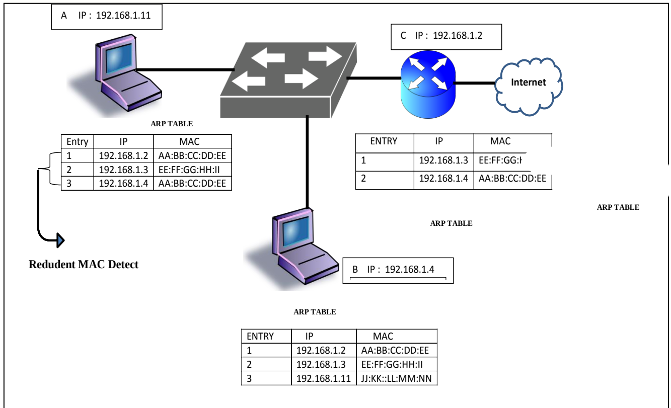
Fig. 3 Detection of ARP spoofing Attack
