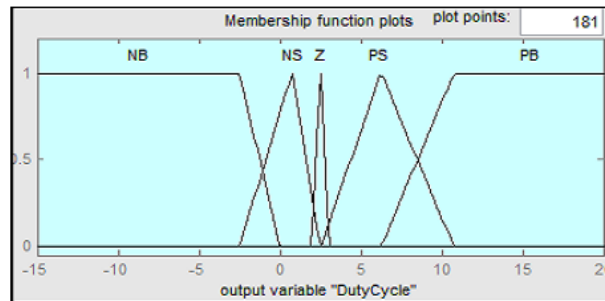
Fig.8. Output variables to defuzzification process
