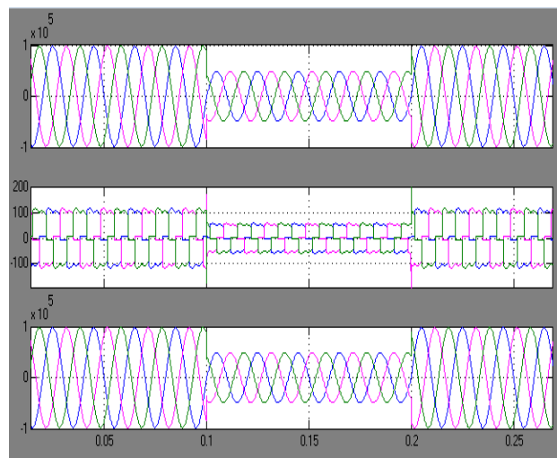
Fig.11. Supply voltage, Load current, load voltage for without UPQC on sag condition.
