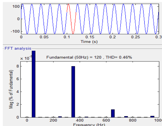
Fig.20. Total harmonic distortion for UPQC with hybrid fuzzy compensated system, THD=0.46%.
