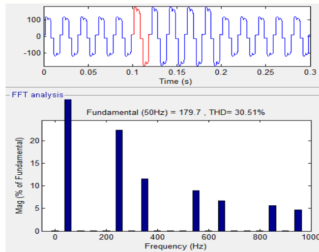
Fig13.Total harmonic distortion for uncompensated system, THD =30.51%
