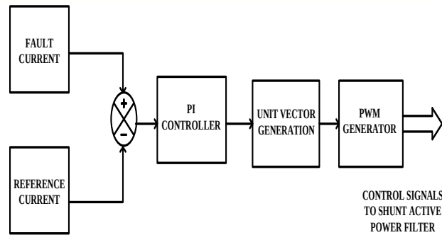
Fig.4. Control strategy for Shunt APF of UPQC.
