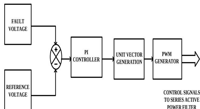
Fig.3. Control strategy for Series APF of UPQC.
