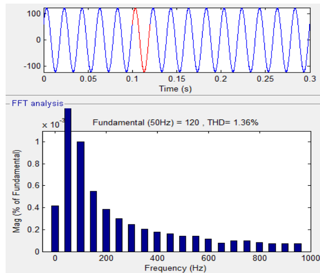
Fig.17. Total harmonic distortion for UPQC with fuzzy compensated system, THD = 1.36%.
