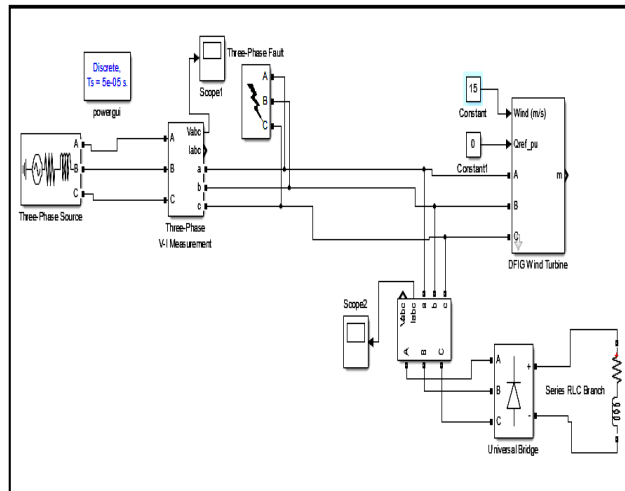
Fig.10. Matlab/Simulink circuit diagram for uncompensated system.
