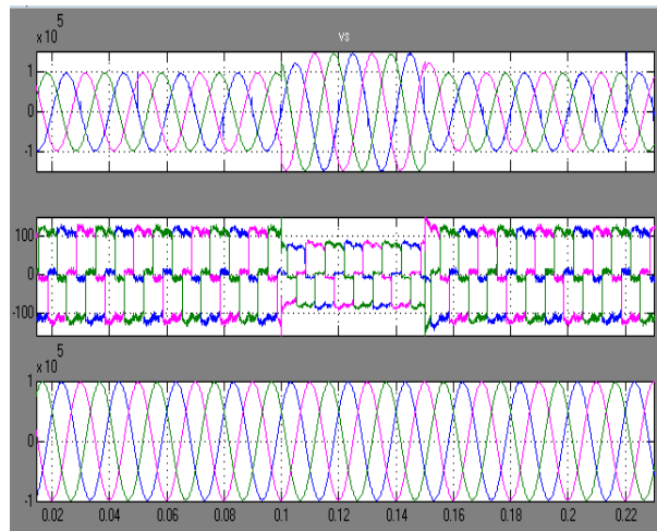
Fig.19. Supply voltage, Load current, load voltage for UPQC with Hybrid Fuzzy Logic Controller on Swell condition.
