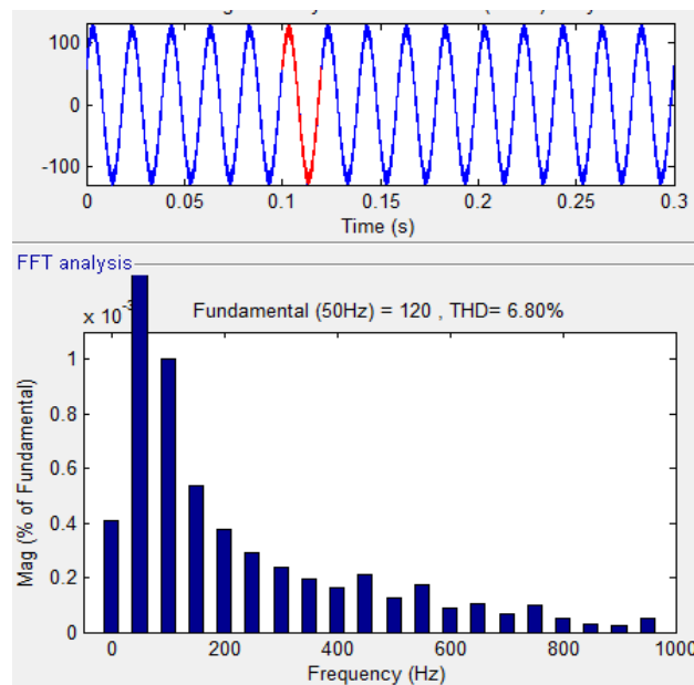
Fig.15.Total harmonic distortion for UPQC compensated system, Base THD =6.80%.
