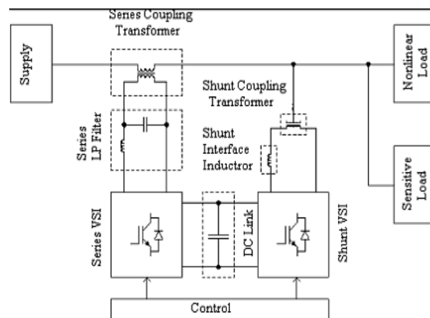
Fig.2. Schematic diagram of Unified Power Quality Conditioner.
