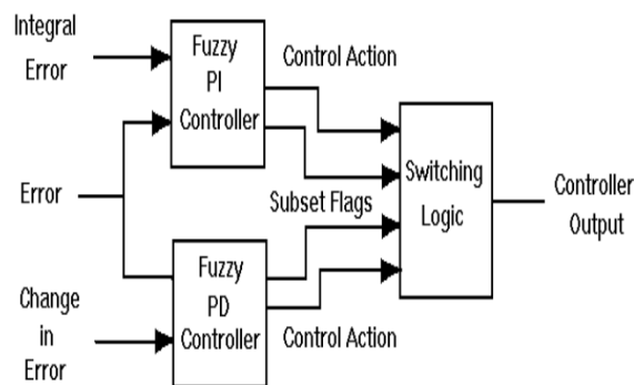
Figure.9. Hybrid Fuzzy PID Controller.
