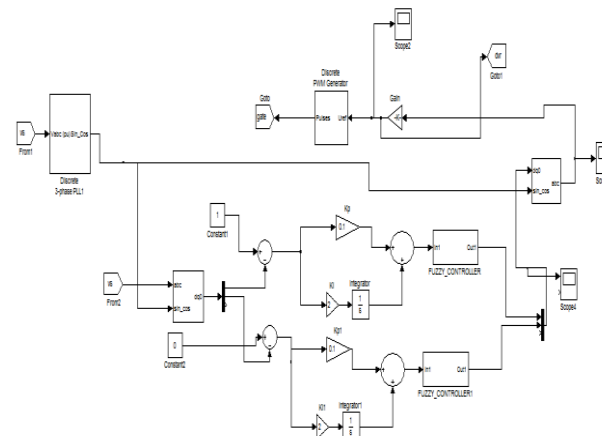
Fig.18. Hybrid Fuzzy logic control block diagram for UPQC system.
