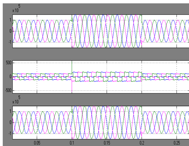
Fig.12. Supply voltage, Load current, load voltage for without UPQC on swell condition
