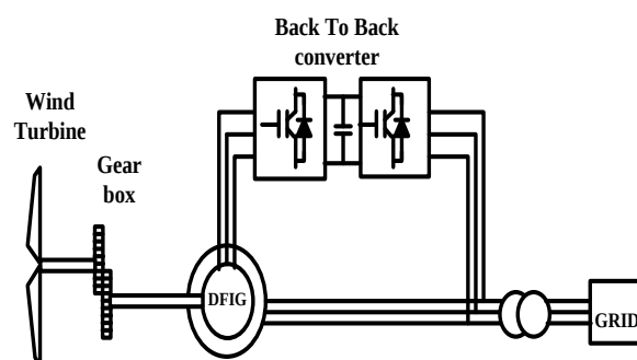
Fig.1. Grid connected DFIG based wind power system.
