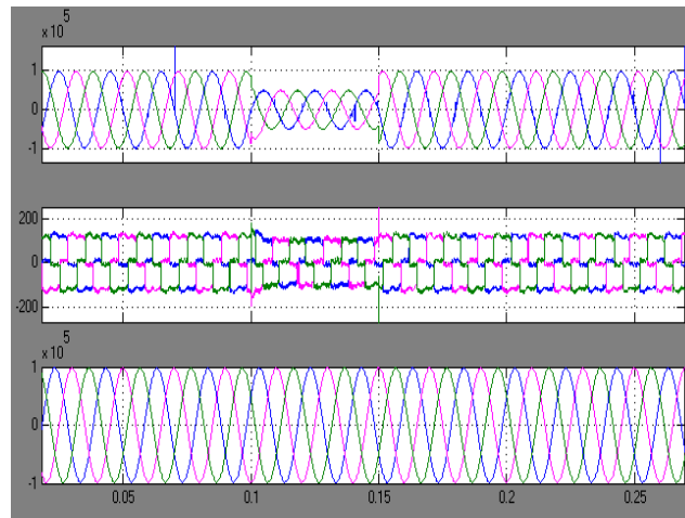
Fig.16. Supply voltage, Load current, load voltage for UPQC with fuzzy on sag condition.
