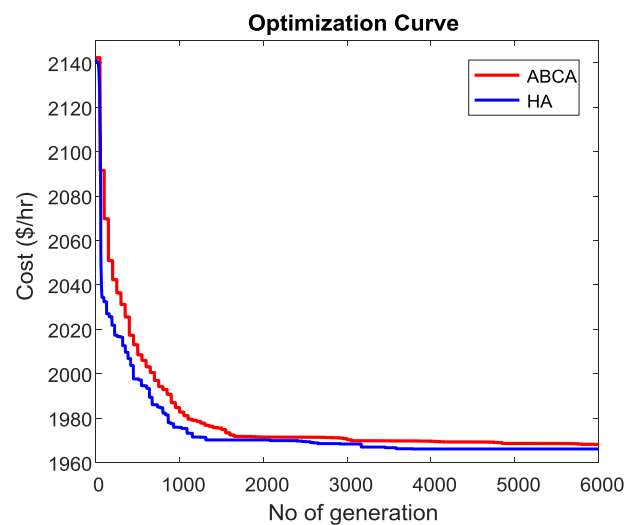
Fig.1.Convergence Characteristics
