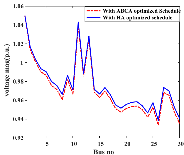
Fig.2. System voltage profile with HA and ABCA optimized schedule
