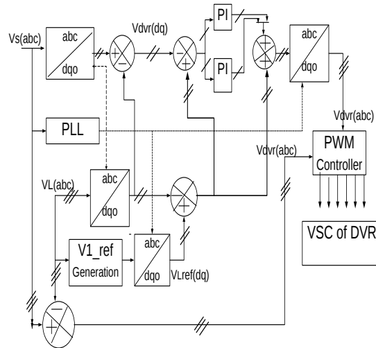
Figure 3: Control Block Diagram for DVR
