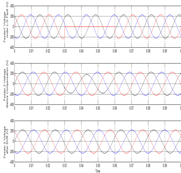
Figure 6: Simulation results for proposed system with PI controller under L-G Fault
