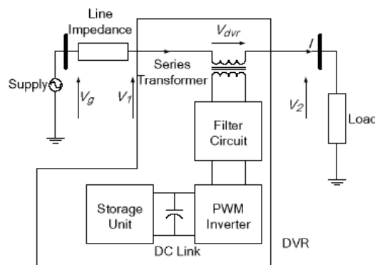
Figure2 Block Diagram of General DVR Circuit
