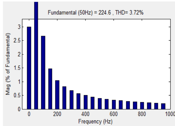
Figure 8: THD for Voltage with PI controller
