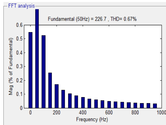
Figure 9: THD for Voltage with ANN controller
