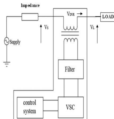
Figure 1: Schematic diagram of DVR
