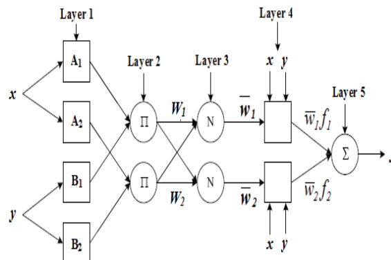
Figure 4: ANN architecture for a two-input multi-layer network
