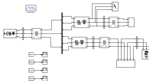
Figure 5: Simulation Diagram for DG system dynamic voltage restorer
