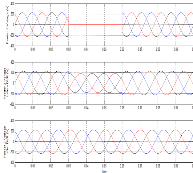
Figure 7: Simulation results for proposed system with PI controller under L-L-L-G Fault
