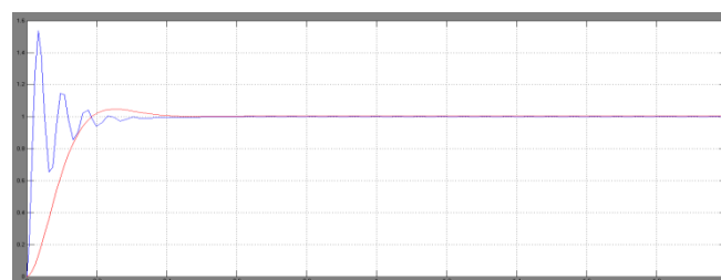
Figure 7: Simulation Result for Speed with Fuzzycontroller
