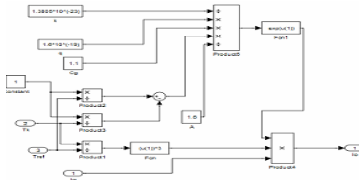
Figure 7: Model takes reverse saturation current, module reference temperature and the module operating temperature as input and calculates module saturation current
