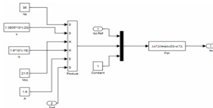
Figure 6: Model for reverse saturation current through the diode
