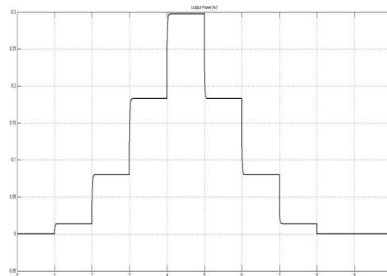
Figure 15: Simulation result for Output Power from BOOST Converter
