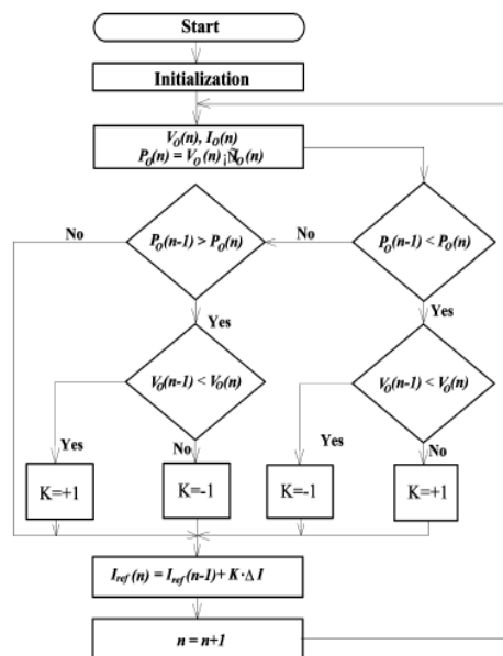
Figure 4: Flow Chart representation of P&O Technique
