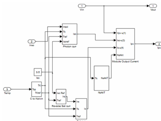
Figure 10: Model contains all the six model interconnected together
