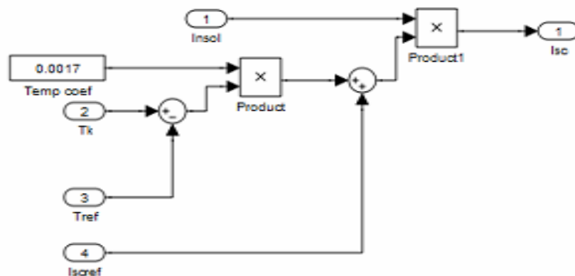
Figure 5: Model for I sc at a given temprature
