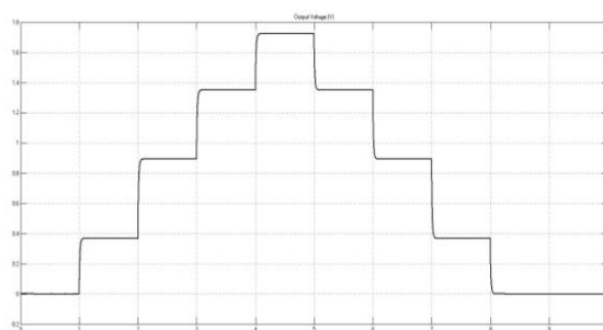
Figure 13: Simulation result for Output Voltage from BOOST Converter
