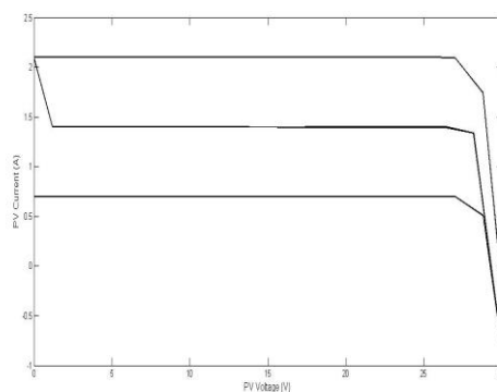
Figure 11: Simulation result for photovoltaic I-V Curve
