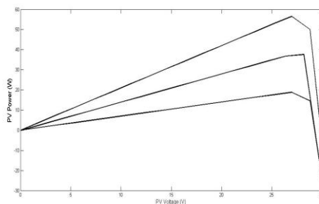
Figure 12: Simulation result for photovoltaic P-V Curve
