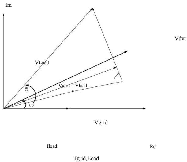
Fig.6. Energy optimization technique
