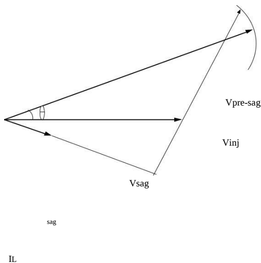
Fig.5. Phase Advance compensation method
