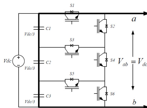
Fig. 2.2.4 Switching configuration required to generate output voltage level IV.
