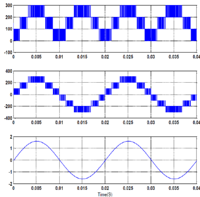
Fig.5. Output voltage of level generator (100 V/div), output voltage (200 V/div) and output current (1 A/div) at M_a=0.8 .(From top)
