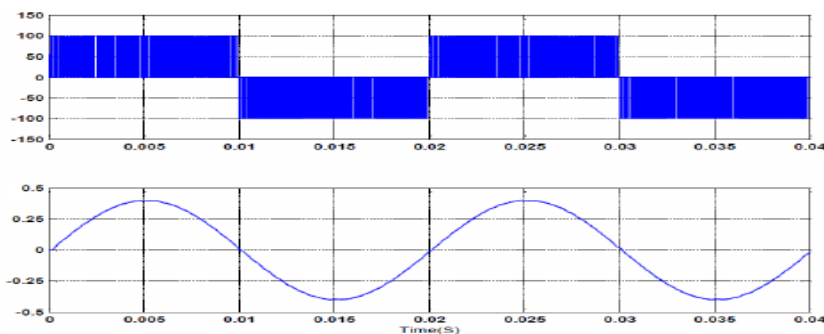
Fig.8. Output voltage of polarity generator (50 V/div), and output current (0.25 A/div) for M_a=0.2 . ( From top)
