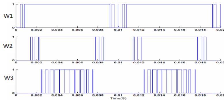
Fig. 4. Decision signals produced by the comparators.
