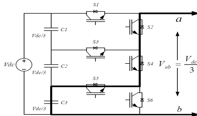
Fig. 2.2.2 Switching configuration required to produce output voltage level 1I.
