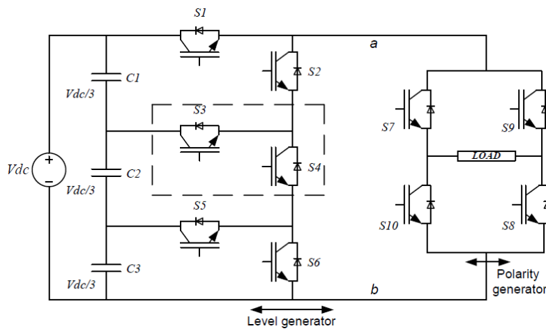
Fig. 2.1 configuration of presented single phase seven-level inverter.
