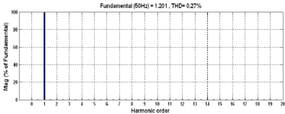
Fig. 7. Current waveform THD for five levels of output voltage of Fig.6.
