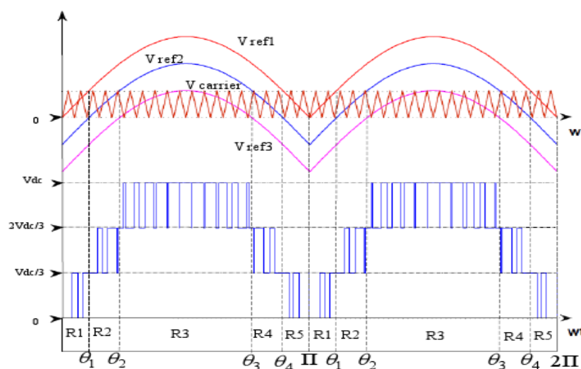
Fig. 3 .From top: PWM switching signal generation, Output of level generator, Output regions for gating signals.
