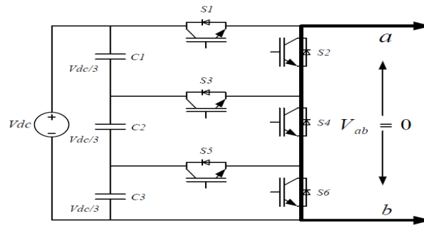
Fig. 2.2.1. Switching sequence required to produce output voltage level I.
