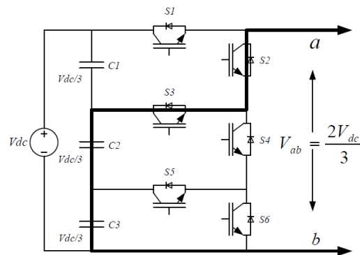
Fig. 2.2.3 Switching configuration required to produce output voltage level III.
