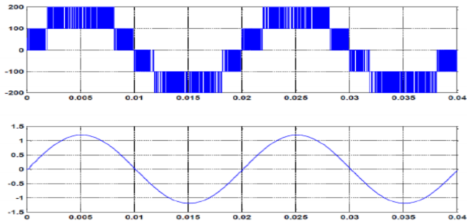
Fig. 6. Output voltage of polarity generator (100 V/div), and output current (0.5 A/div) for M_a=0.6 (From top)
