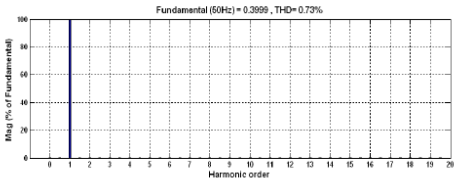
Fig. 9. Current waveform THD for three levels of output voltage of Fig.8
