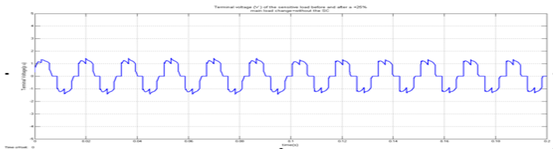
Fig 3: Terminal voltage (V) of the sensitive load before and after a 25% main load change: without SC
