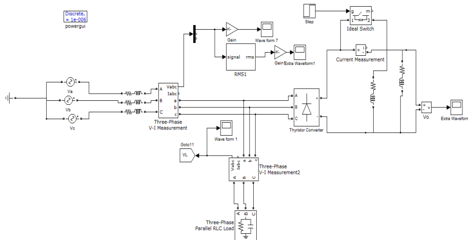
Fig 2: Isolated Power System without Series Compensator
