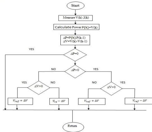
Figure3. Flow chart for MPPT algorithm.
