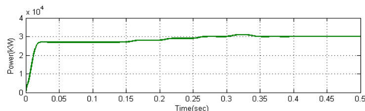
Figure12. Output power of doubly fed induction generator
