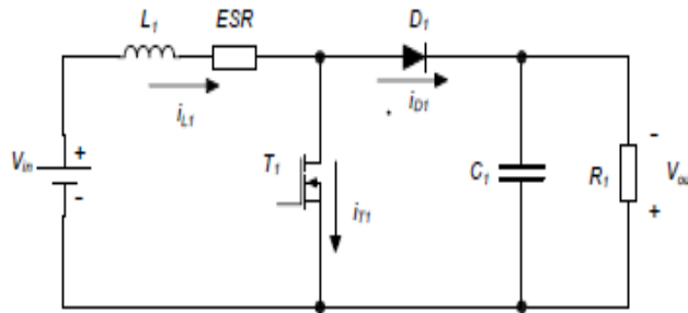
Figure 4. Boost Converter
