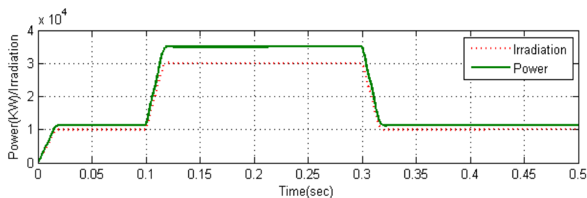
Figure 9. PV output power and sola irradiation
