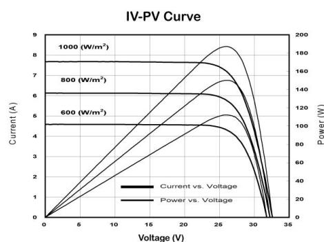
Fig.5. I-V and P-V Characteristics of PV Array
