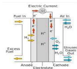
Fig.7.schematic diagram of fuel cell
