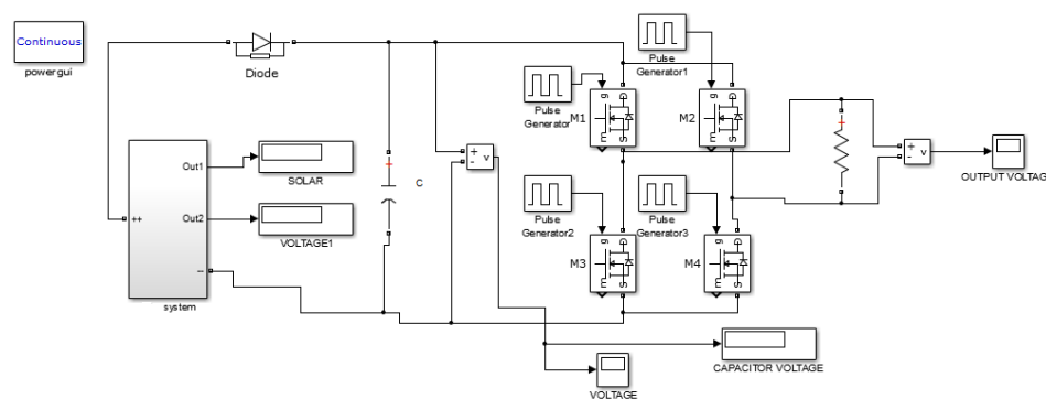
Fig.9. simulink diagram of proposed system
