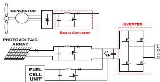
FIG.1. Proposed model of hybrid system
