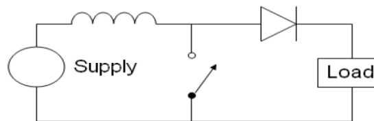
Fig.8.schematic diagram of boost converter
