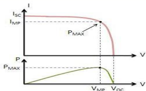
Fig.4. Output characteristics of PV Array
