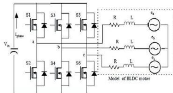
Fig. 2: Mathematical model of BLDC motor
