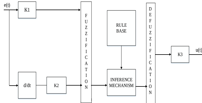
Figure 6: basic structure of fuzzy logic controller
