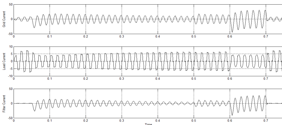
Figure 8: Waveforms for (a) Source Current. (b) Non-Linear Load current. (c) APF current with fuzzy controller
