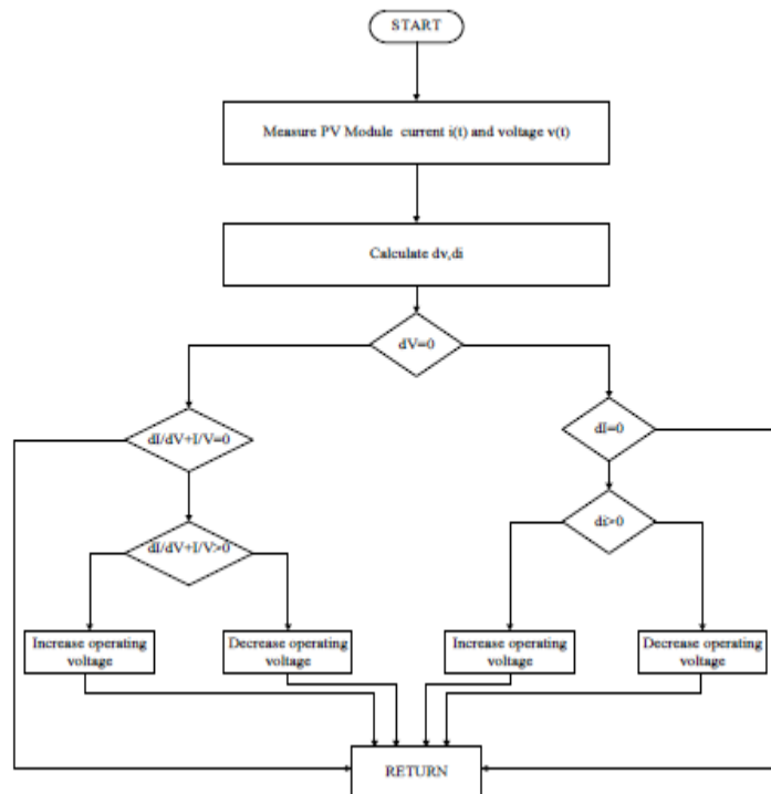
Figure 5: INC MPPT flow chart
