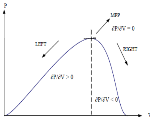
Figure 4: Characteristics of PV Power Vs Voltage under INC method
