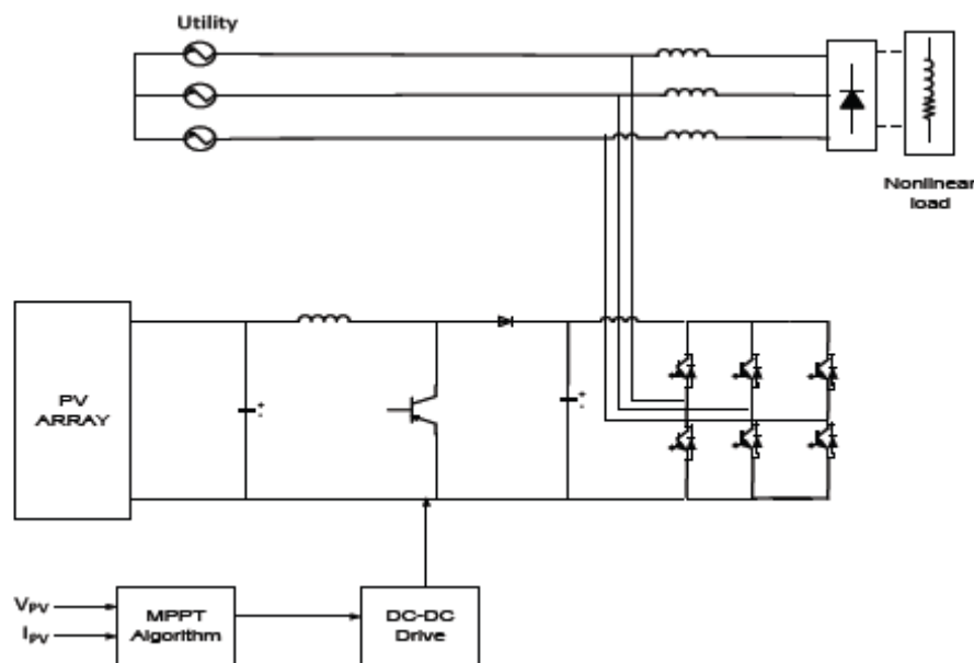
Figure 1: Configuration of Proposed Grid Connected PV-APF System
