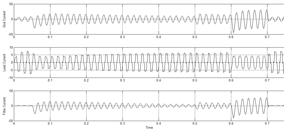
Figure 7: Waveforms for (a) Source Current. (b) Non-Linear Load current. (c) APF current with PI controller
