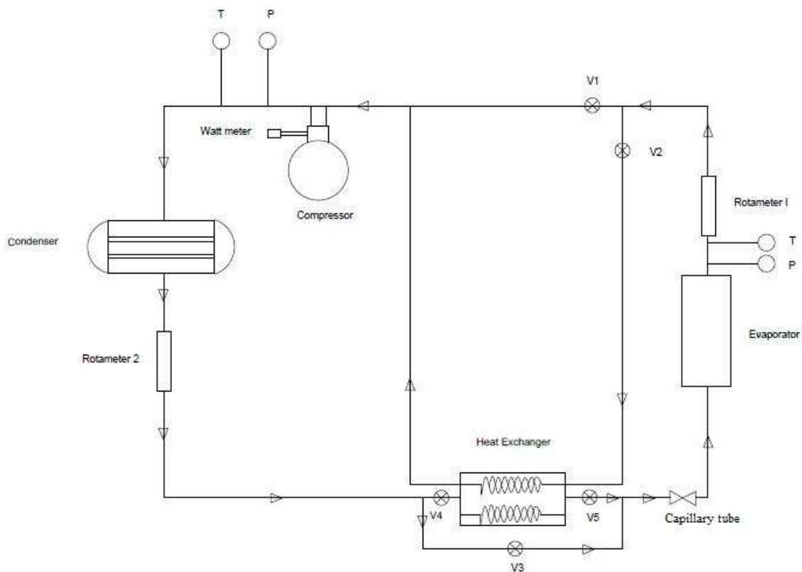
Fig. 1 Schematic diagram of domestic refrigerator experimental setup.
