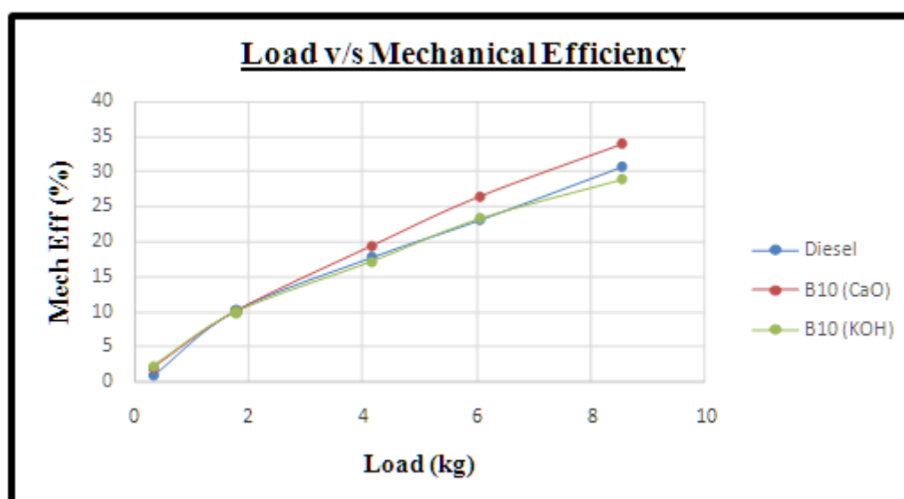
Fig 2. Load v/s Mechanical Efficiency
