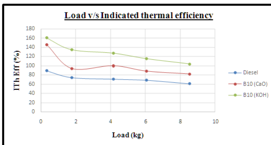
Fig 4. Load v/s Indicated Thermal Efficiency
