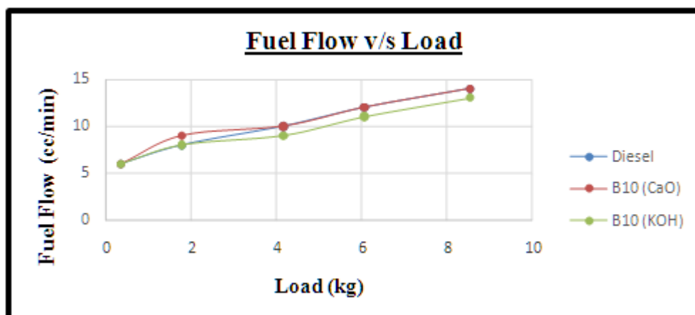
Fig 5. Load v/s Fuel Flow
