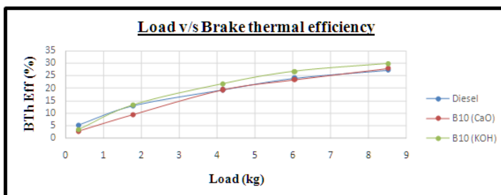
Fig 1. Load v/s Brake Thermal Efficiency
